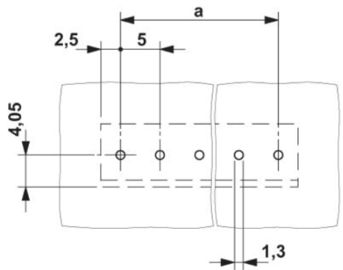
Drilling diagram
